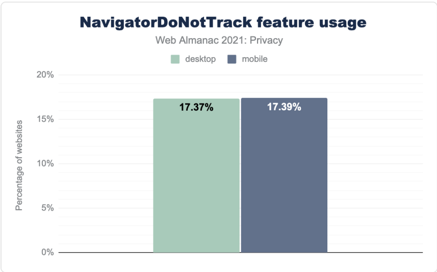
Figure 11.27. Percentage of websites using Do Not Track (DNT).
