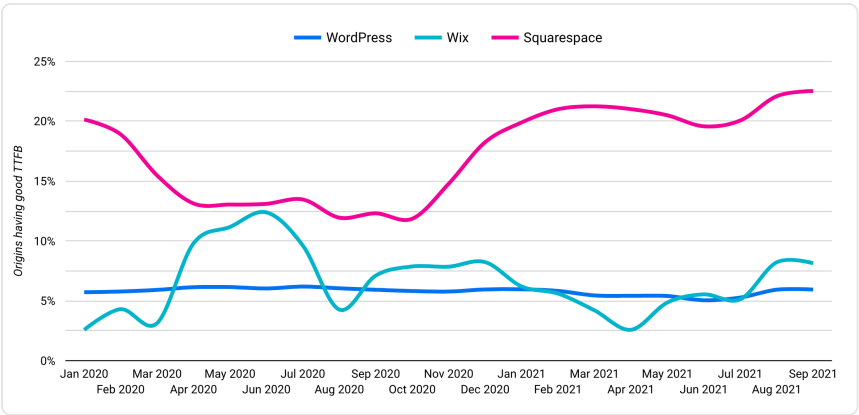
Figure 10.11. Origins having good TTFB by CMS (Core Web Vitals Technology Report 421 )
