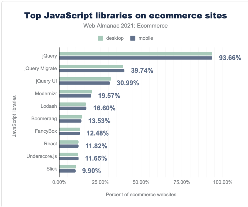
Figure 17.28. Top JavaScript libraries on ecommerce sites.
