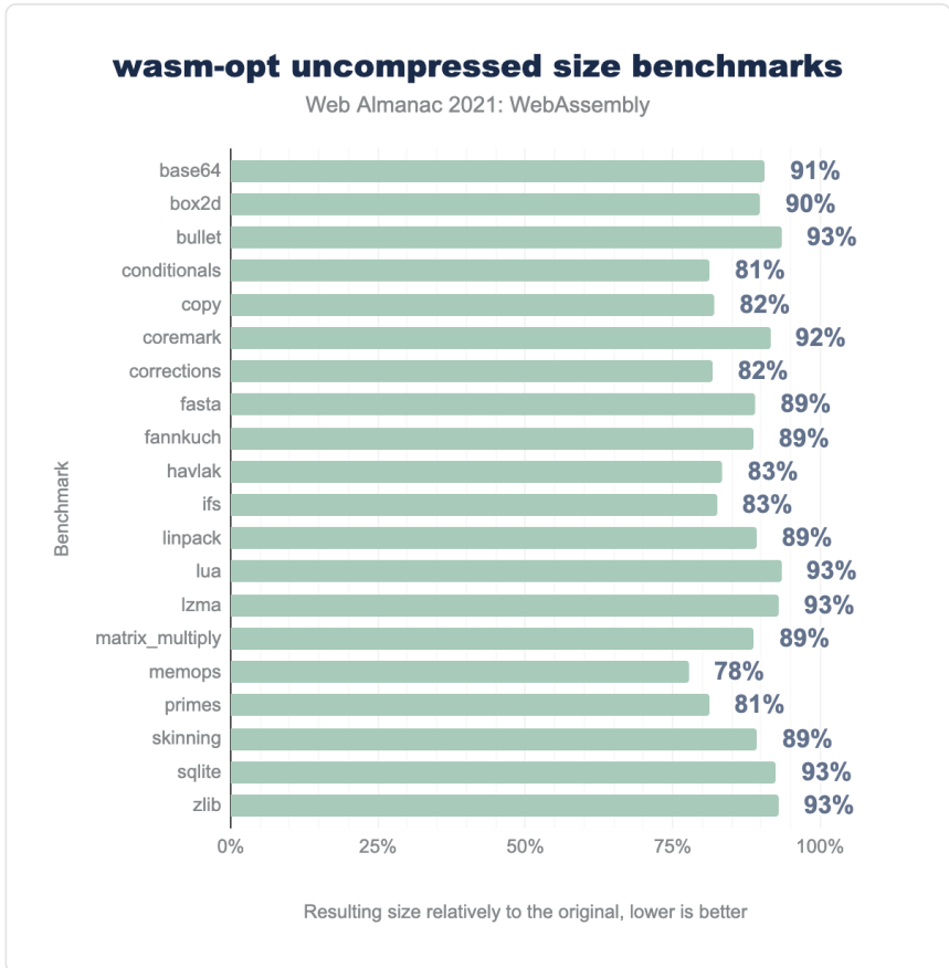
Figure 6.17. wasm-opt uncompressed size benchmarks.
