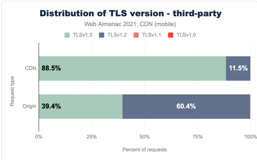
Figure 21.11. Distribution of TLS version for third-party requests (mobile).
