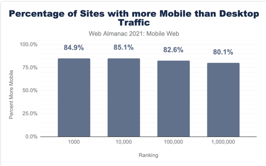
Figure 13.2. Percentage of Sites with more mobile than desktop traffic.
