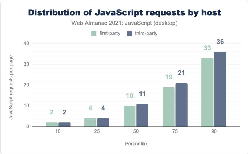
Figure 2.12. Distribution of the number of JavaScript requests per desktop page by host.
